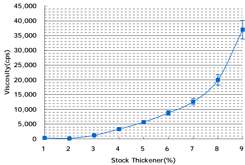
SEATEX S-9 粘度曲线
