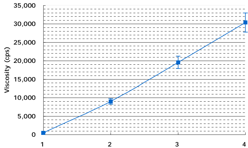
SEATEX MGB400 粘度曲线
