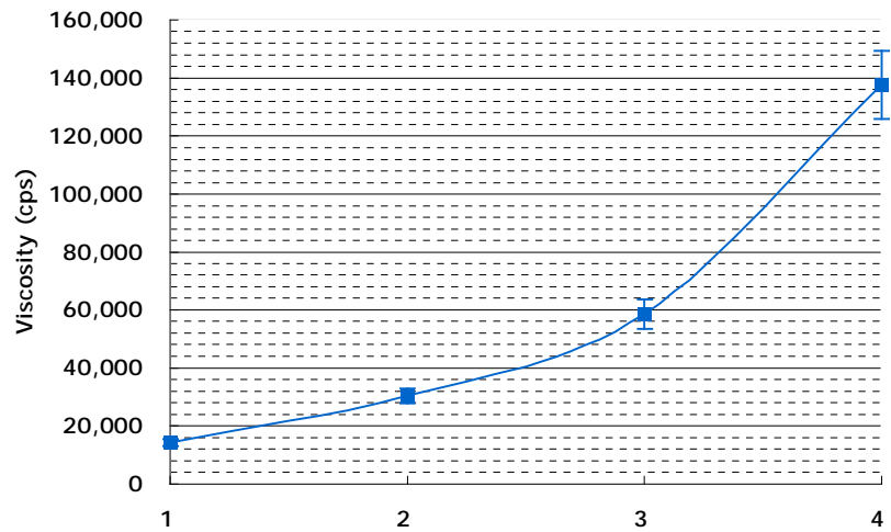
SEATEX MGB200 粘度曲线
