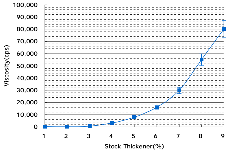
SEATEX GPN 粘度曲线
