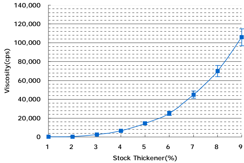
SEATEX GP50 粘度曲线
