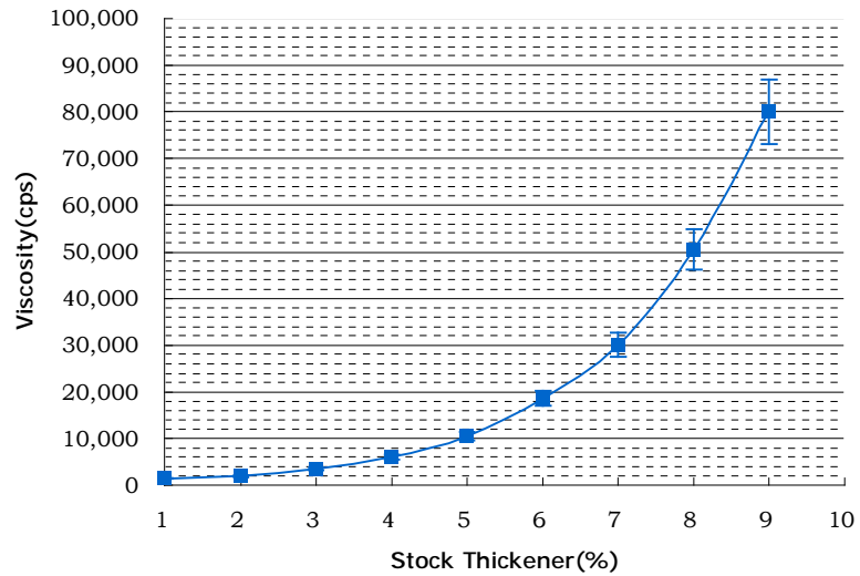
SEATEX CD 粘度曲线
